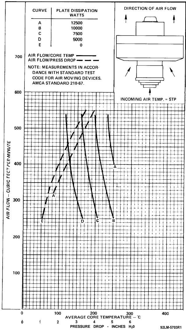
Figure 5 - Air Flow Characteristics
